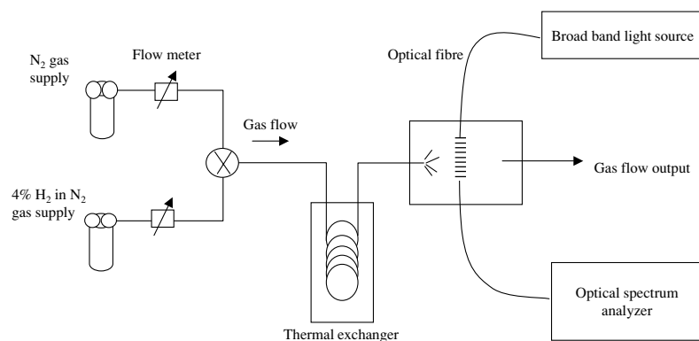
Figure 1. Experimental set-up.
