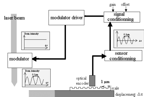
Fig. 4. Exposure beam intensity control loop
