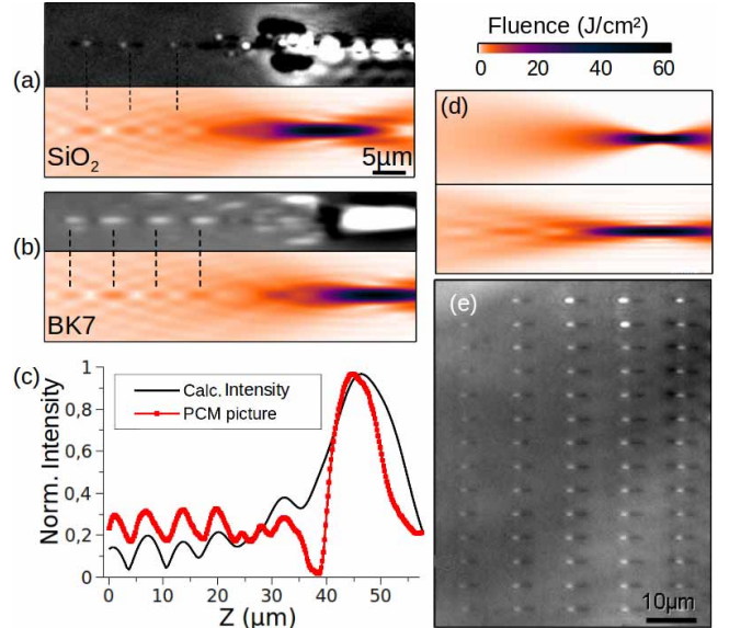
Fig. 2. (a), (b) PCM pictures of single pulse irradiation effects in FS and BK7 with the Fresnel propagation results with NA = 0.45 and T = 1 . The dashed lines shows the correspondence between the position of the dots and the calculated fluence peaks. (c) Horizontal section of the PCM picture (red) and of the numerical results (black) for BK7. (d) Calculated focusing of a pure (top) and truncated (bottom) Gaussian beam showing fluence peaks before the focus due to truncation. (e) Array of dots written in FS in this regime. Each line was written with a single pulse. The main damage (not shown) is situated on the right.
