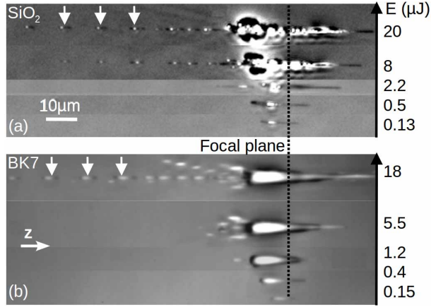
Fig. 1. PCM pictures of single pulse irradiation effects in FS and BK7 at different pulse energies ( E ) with NA = 0.45 and T = 1 . The laser propagates along z . For sufficient energy, a particular photowriting regime occurs where regularly spaced dots appear up to 200 \mu\text{m} before the focus area upon single pulse in both glasses.
