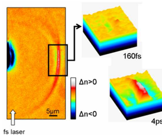
Fig. 3: Pressure wave picturing from PCM images for various pulse duration in fused silica at constant pulse energy. (4.3 μJ, NA= 0.45 )
