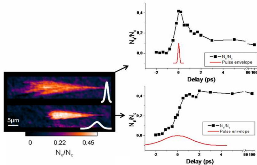
Fig 4. Calculated transient electronic density for single irradiation with (top) a 150 fs pulse and (middle) a 3 ps pulse. Each irradiation sequence carries 6 \mu\text{J} . Left column: example of the N_e/N_c 2D map corresponding to the delay of maximum free carrier generation. Right column: temporal evolution of the maximum N_e/N_c with indication of the irradiation envelope. Laser comes from left.
