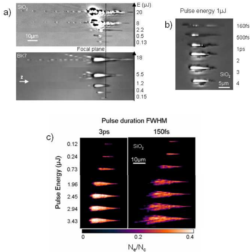
Fig. 2 Comparison of single femtosecond and picosecond irradiation from permanent and transient modifications in fused silica and BK7 glass. a). PCM pictures of single short pulse irradiation effects in fused silica and BK7 glass at different pulse energies (E). The laser propagates along z. For both glasses, the permanently modified volume extends around the focal plane increasingly with the pulse energy. b) Effect of the pulse duration in fused silica. c) Intensity dependence of the transient electronic density N_e normalized to N_{cr} for femtosecond and picosecond pulse. The N_e/N_{cr} mapping is calculated from optical transmission microscopy pictures.
