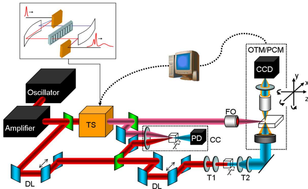
Fig. 1. Experimental set up. TS: temporal shaper illustrated in the top inset. FO: focusing objective. OTM-PCM: Optical transmission and phase contrast microscopy \chi^2 : Frequency doubling crystal. PD: Photodiode. CC: Cross-correlation apparatus. DL: delay line. T1, T2: Telescopes.
