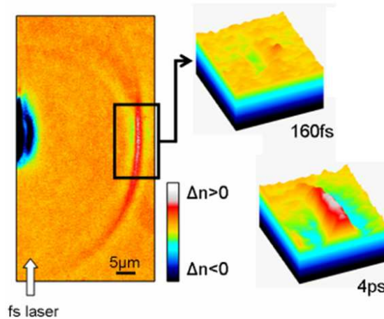
Fig. 3: Pressure wave picturing from PCM images for various pulse duration in fused silica at constant pulse energy. (4.3 \mu J, NA= 0.45 )
