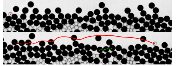
Fig. 1. Example of trajectories for two tracked beads (cropped images). Green color is for a coarse black bead and red is for a smaller transparent bead.
