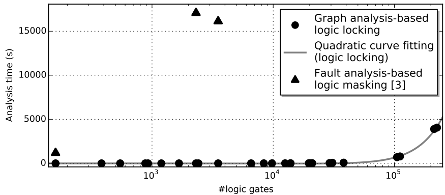
Fig. 13 Time required to analyze and modify the netlist
